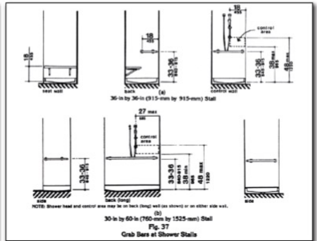
Accessible Shower Stall Grab Bars and Seat, Shower, and Control Area
